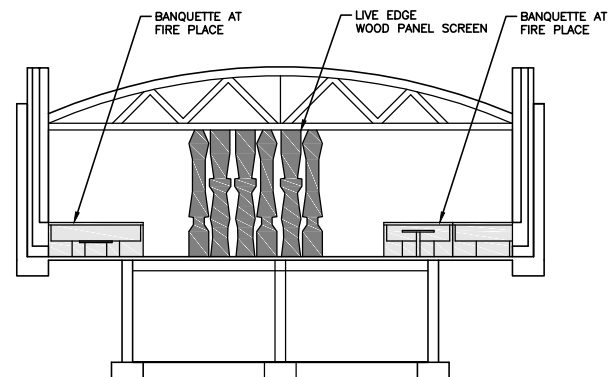
05 SECTION PROPOSED A100 1/8"=1'-0"
