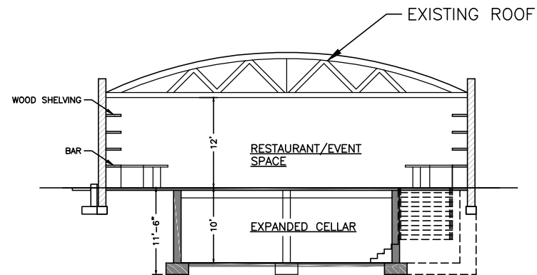
04 SECTION PROPOSED A100 1/8"=1'-0"
