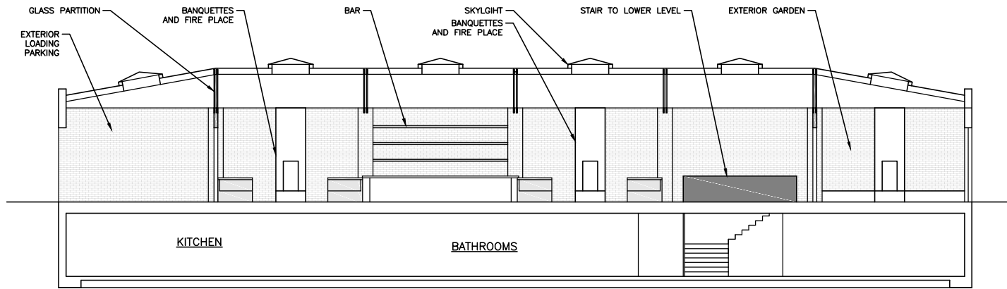
03 SECTION PROPOSED A100 1/8"=1'-0"
