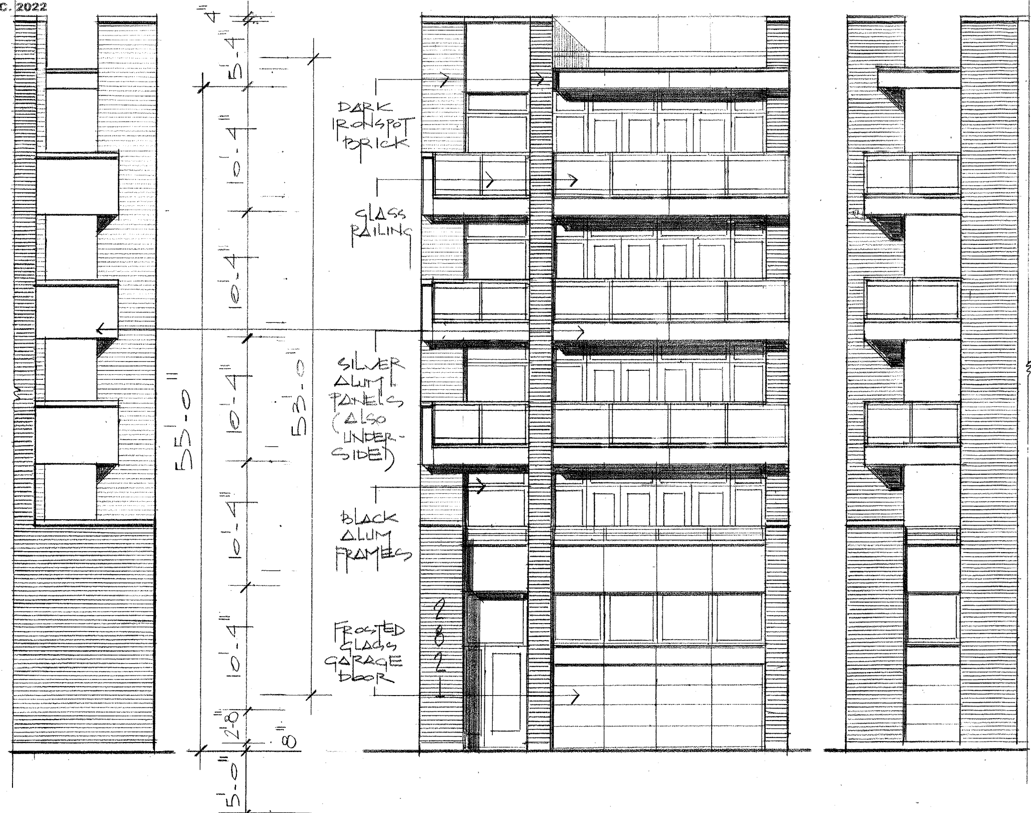
○ NORTH VIEW \frac{1}{8}'' = 1'-0'' ○ FRONT ELEVATION \frac{1}{8}'' = 1'-0'' ○ SOUTH VIEW \frac{1}{8}'' = 1'-0''
