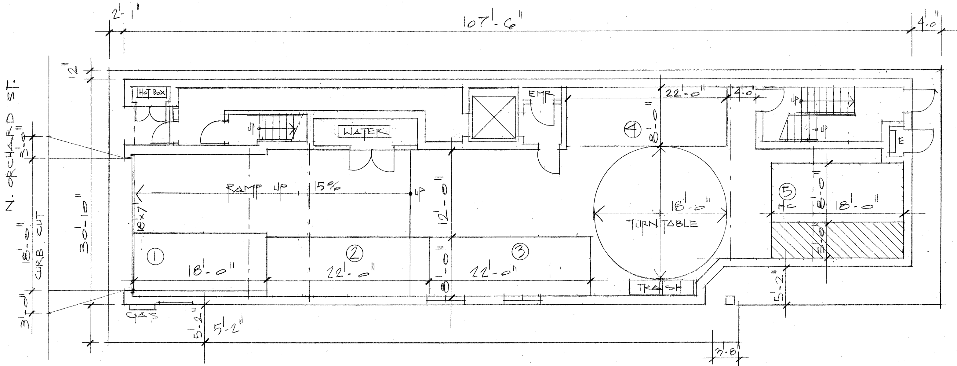
○ BASEMENT FLOOR PLAN 1/8" = 1'-0"
