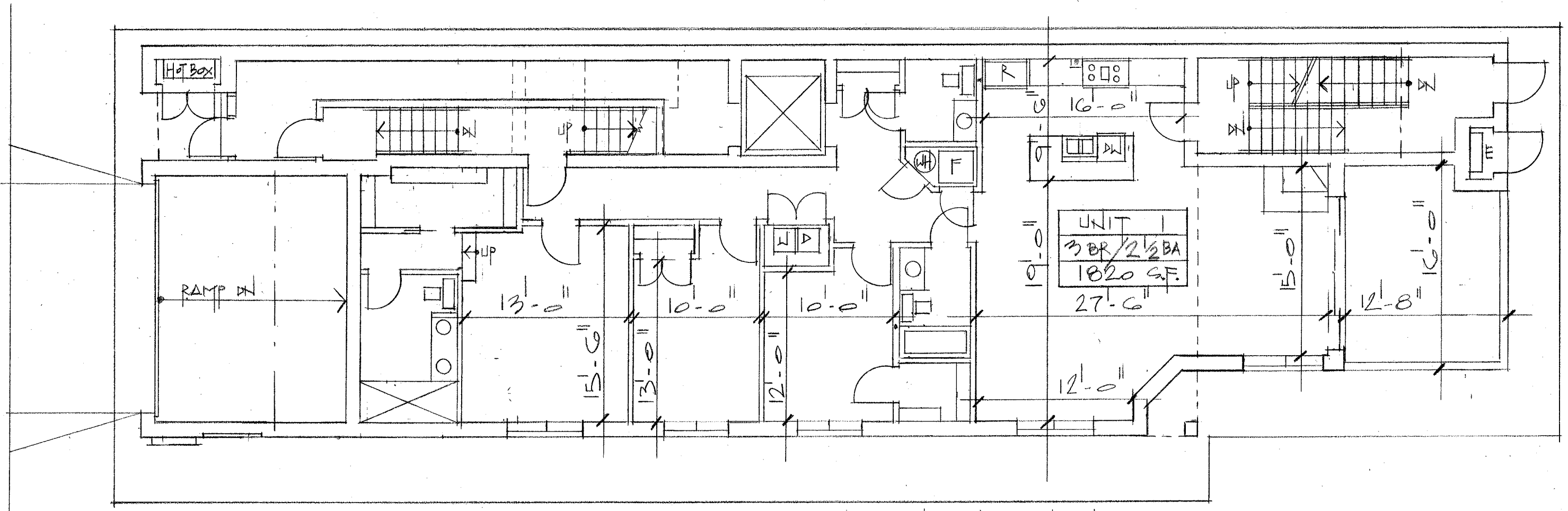
1st FLOOR PLAN 2,575 S.F. 1/8" = 1'-0"
