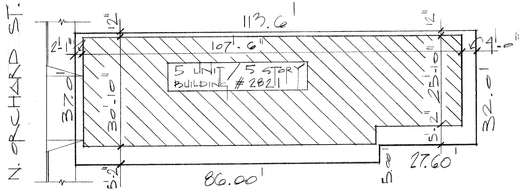
⊕ SITE PLAN 1/16" = 1'-0"
