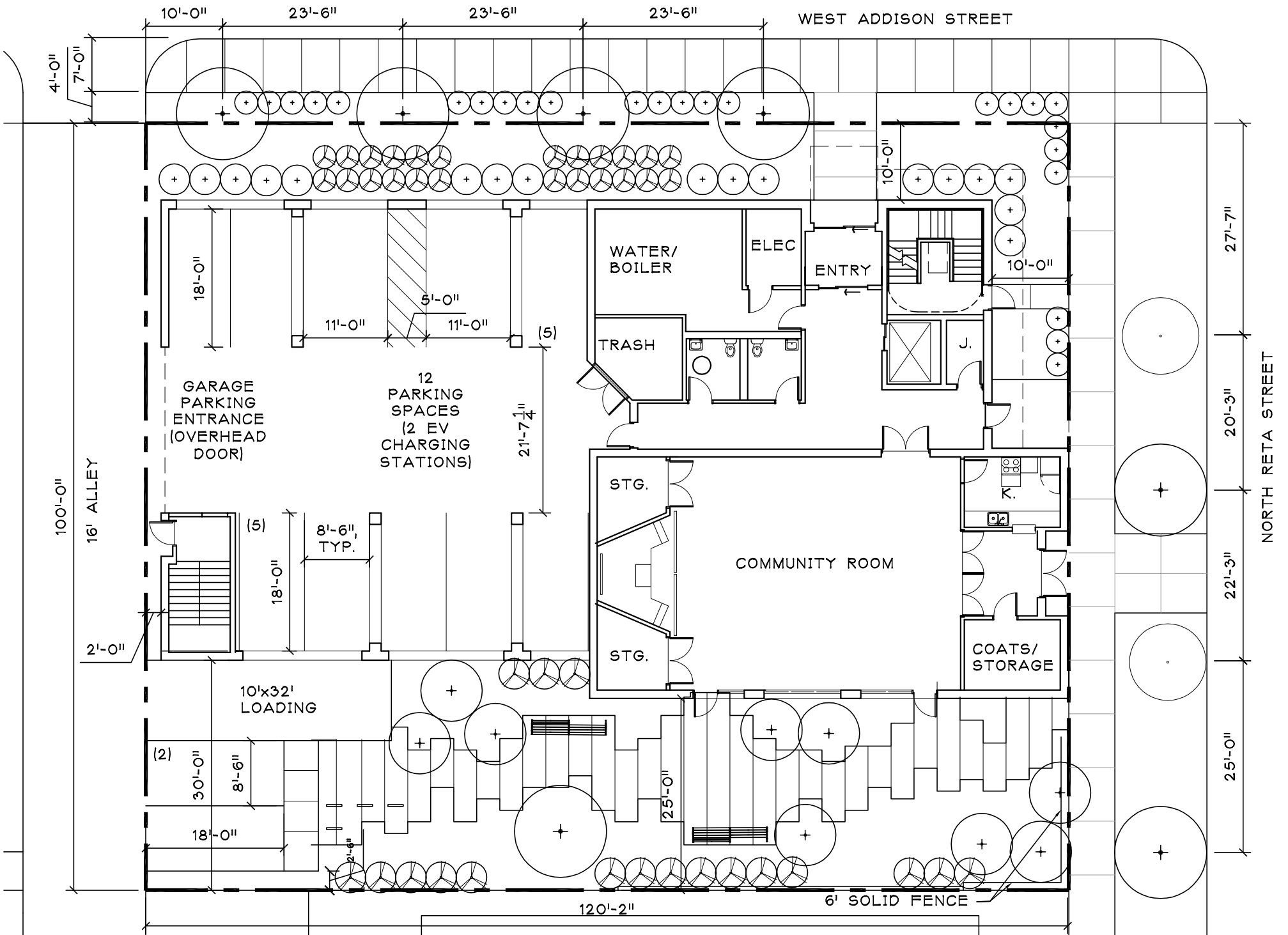
SITE PLAN/GROUND FLOOR PLAN
