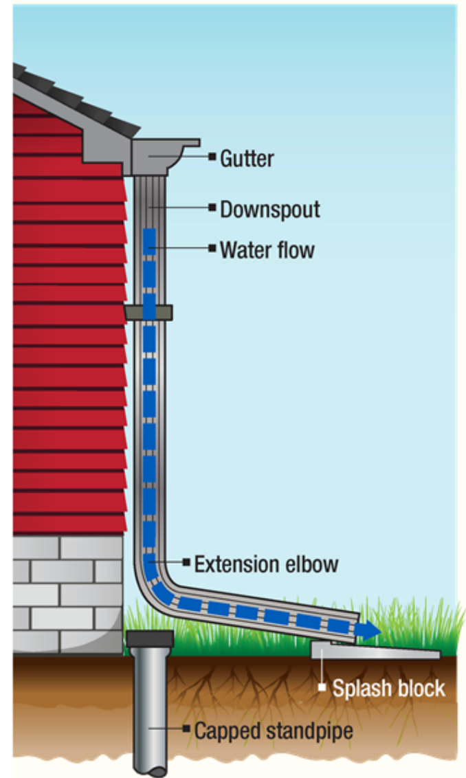
Downspout disconnected from the sewer system
