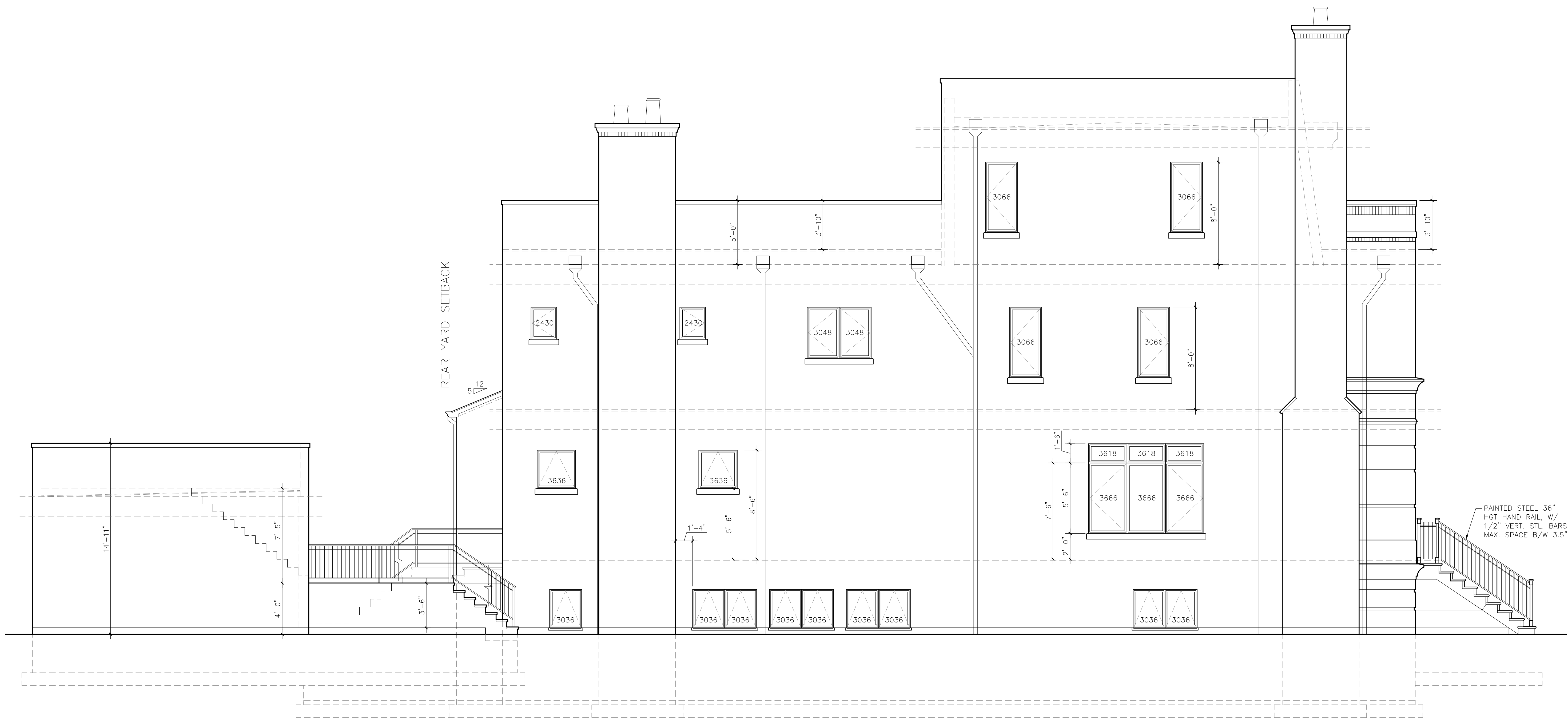
1 SOUTH ELEVATION SCALE: 1/4" = 1'-0"
