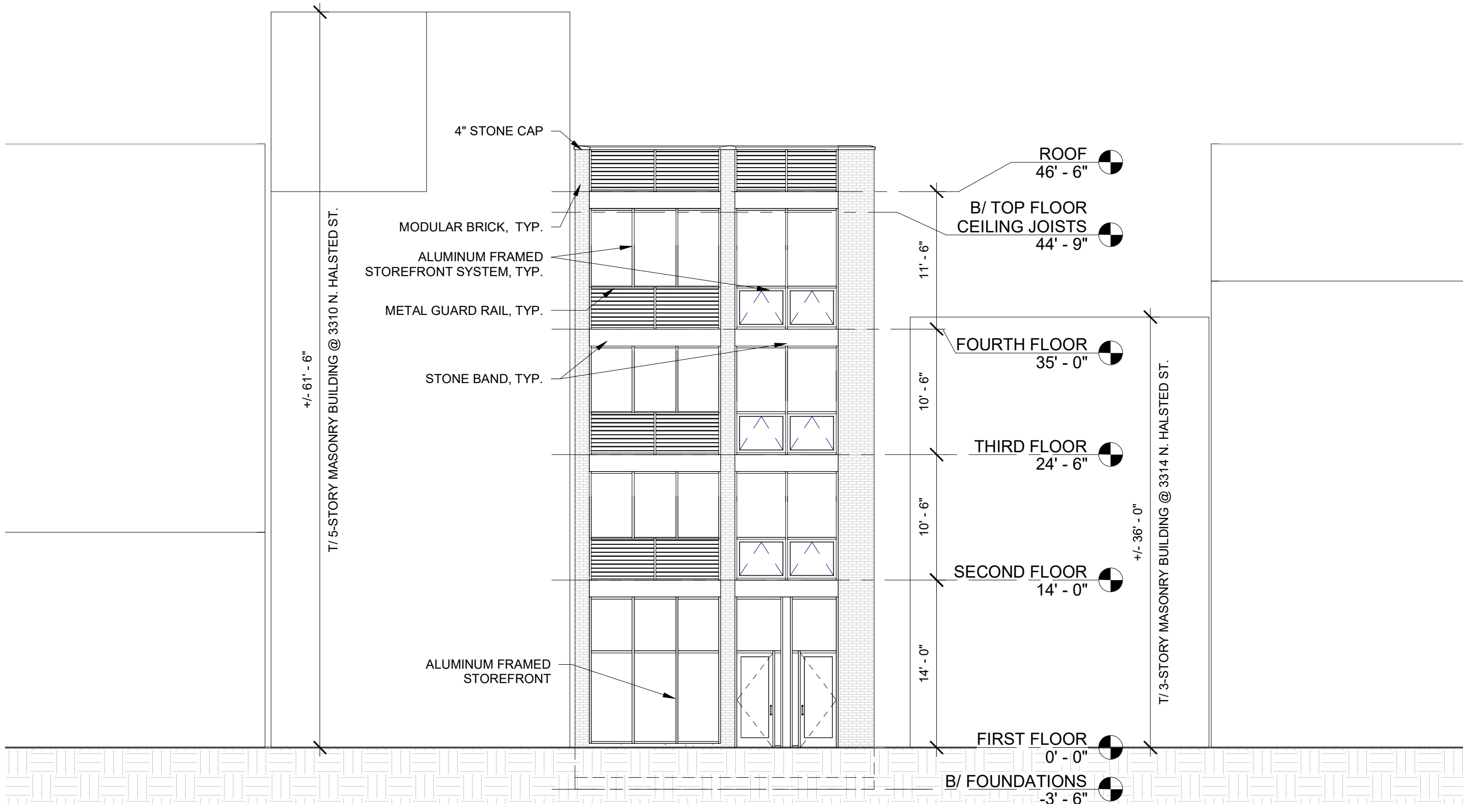
1 EAST ELEVATION 1/8" = 1'-0"
