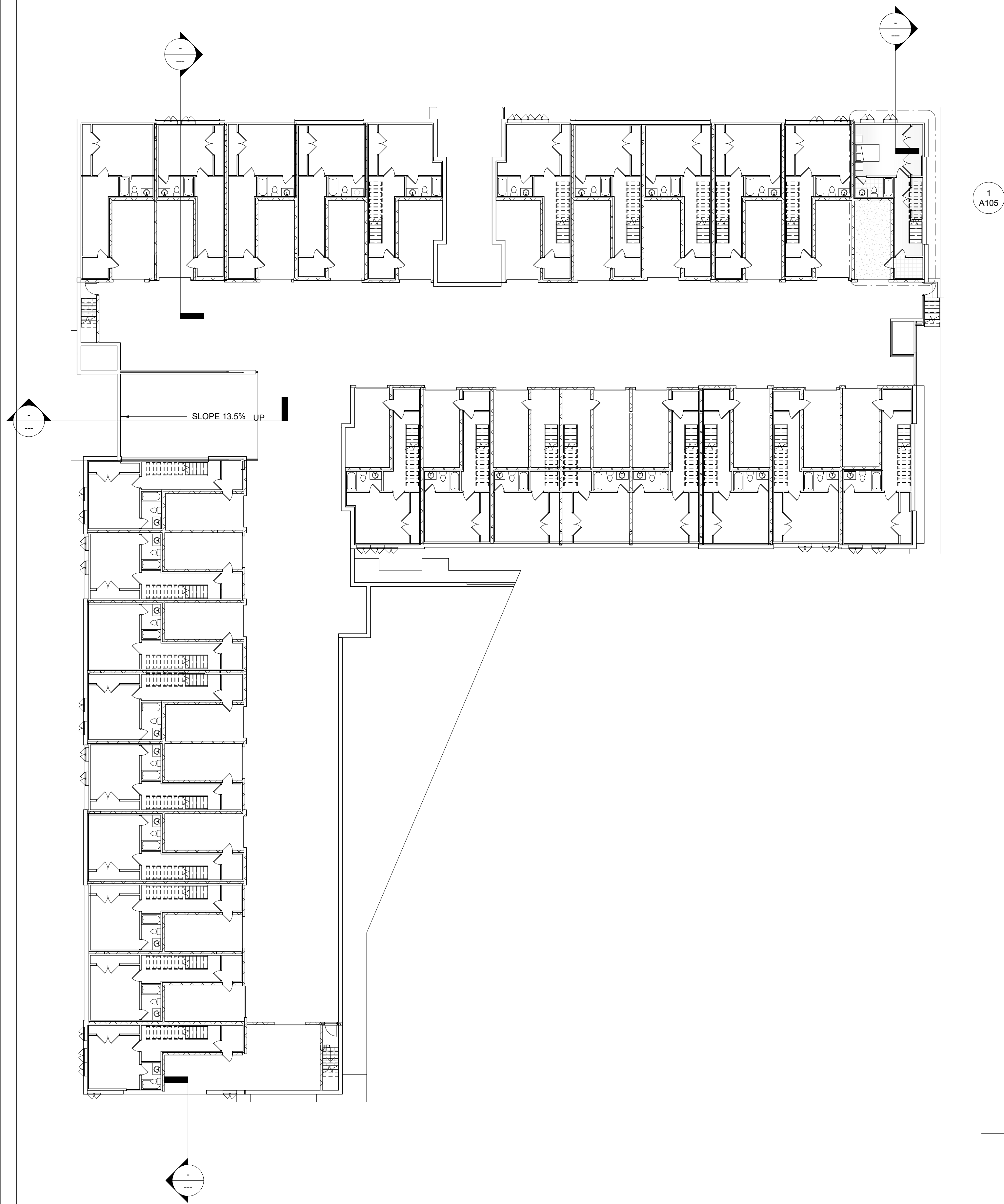
2 1-BASEMENT 1/16" = 1'-0"
