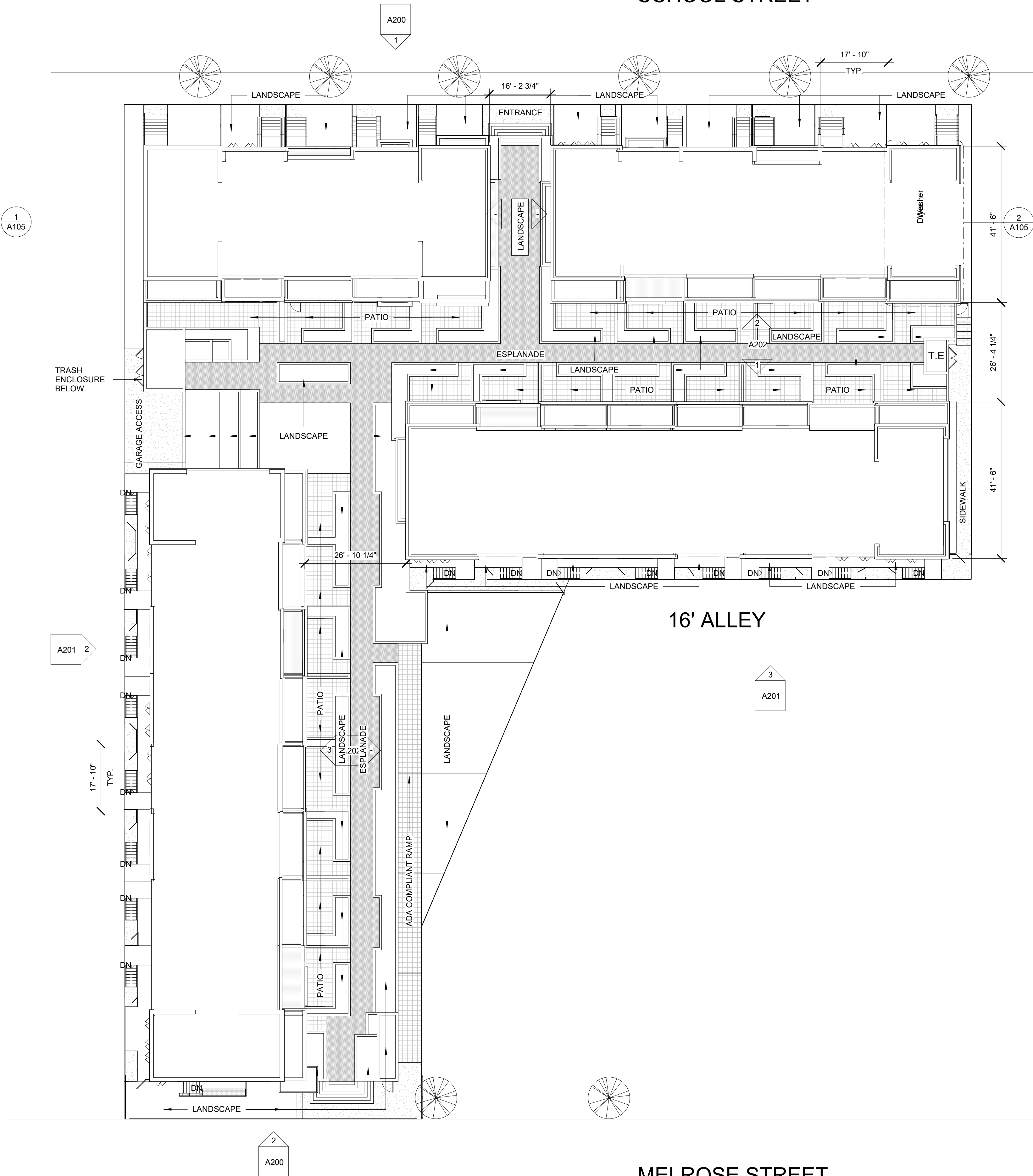
1 2-1ST FLOOR 1/16" = 1'-0"
