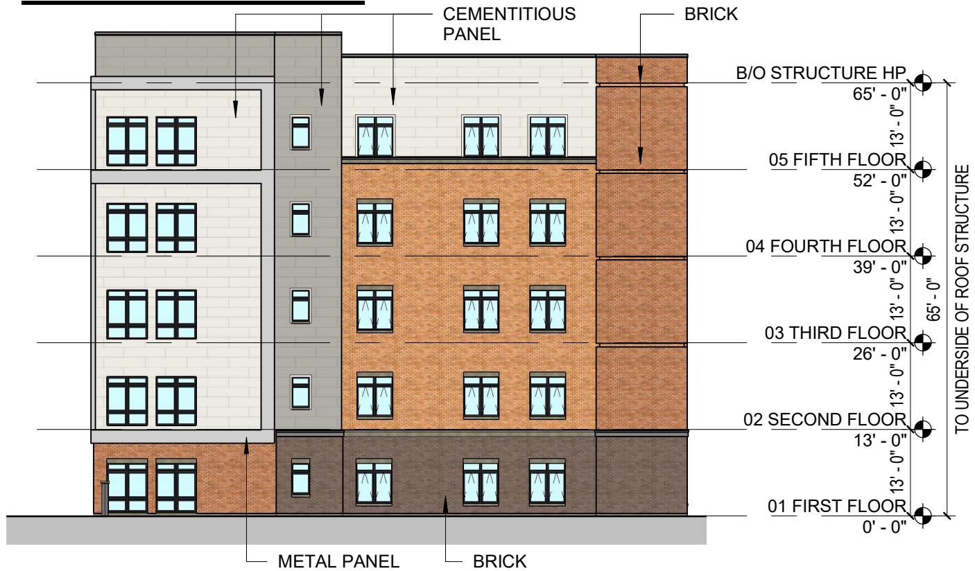
NORTH ELEVATION
