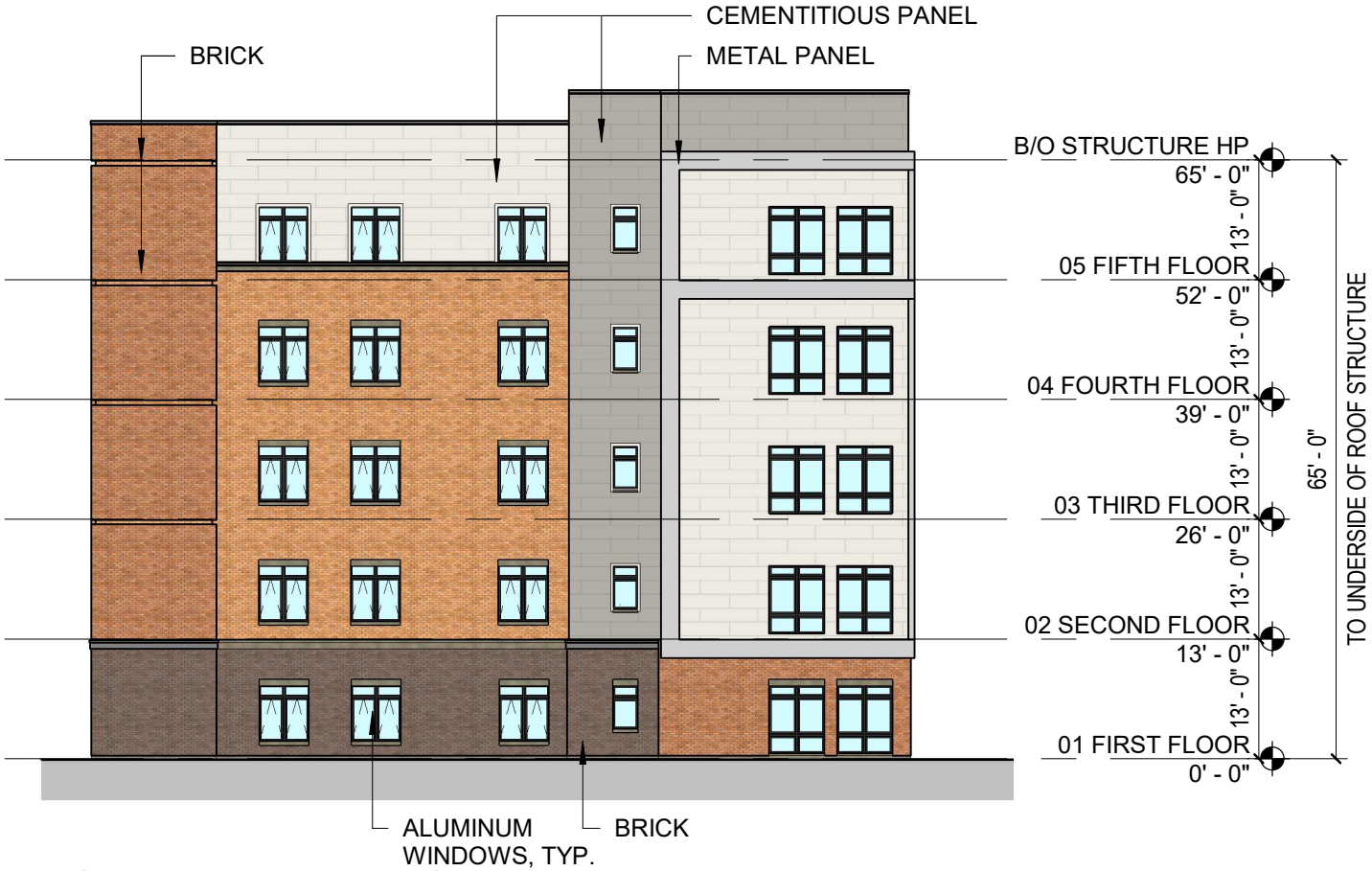
NORTH ELEVATION
