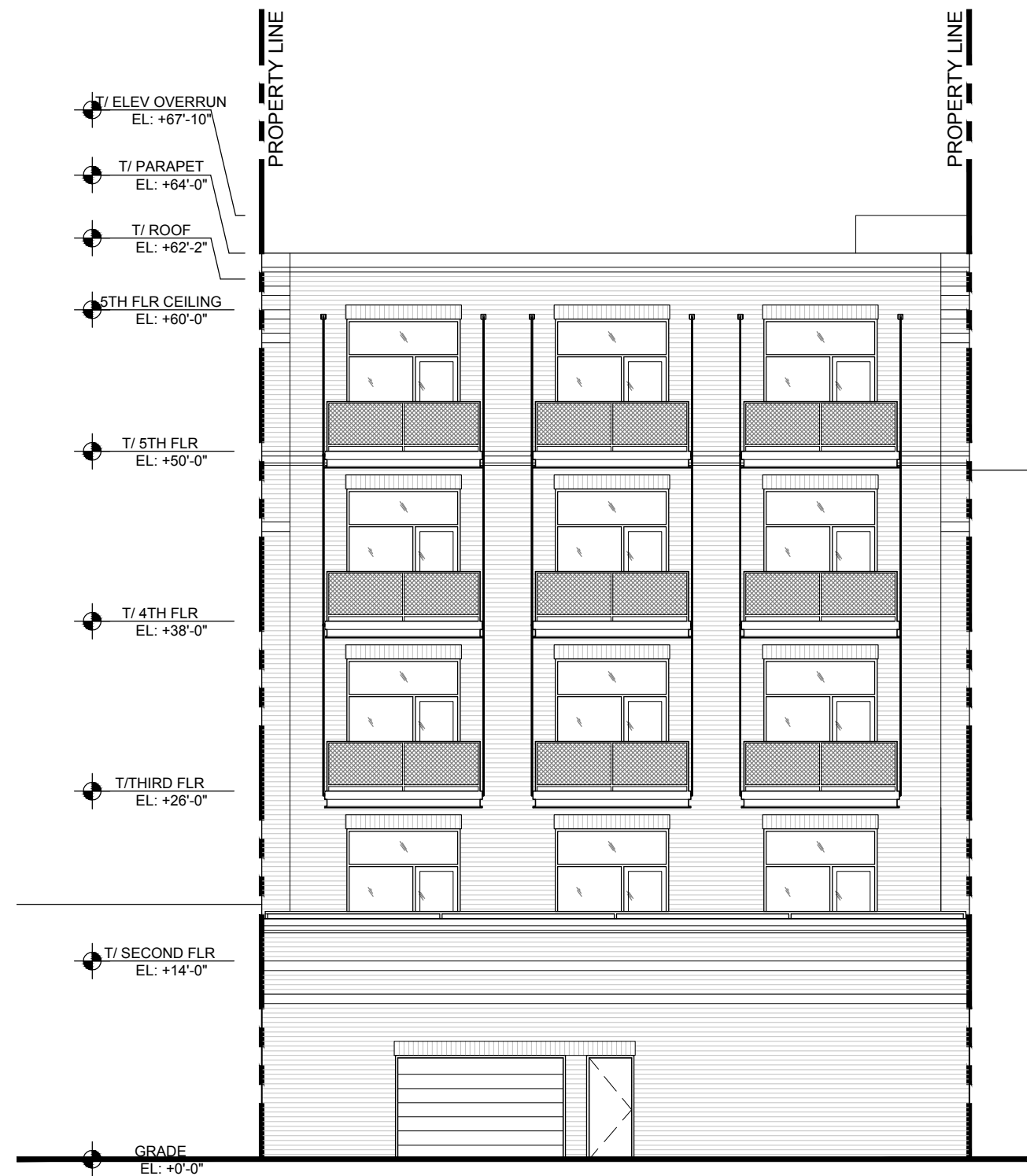
EAST ELEVATION
