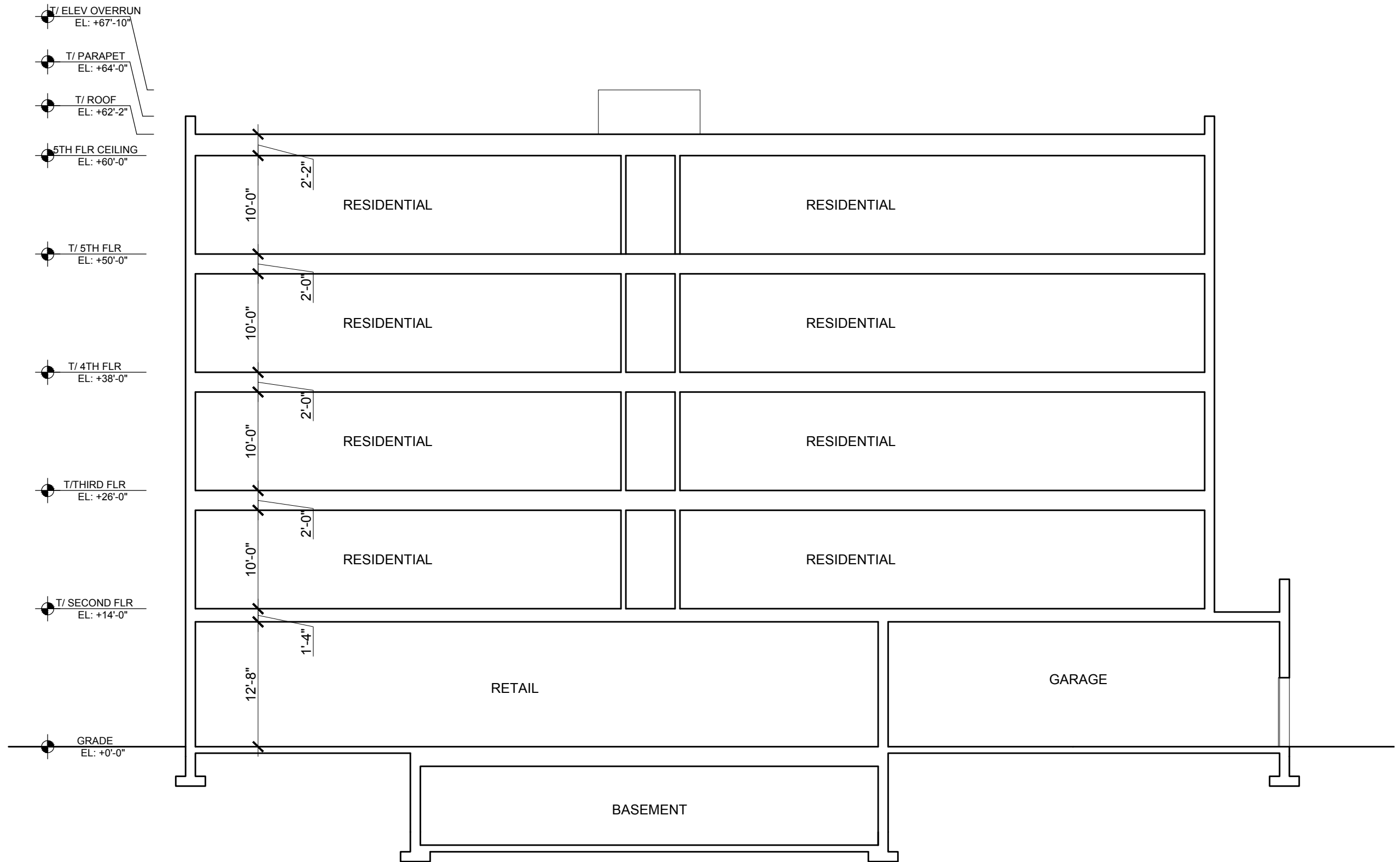
SECTION
