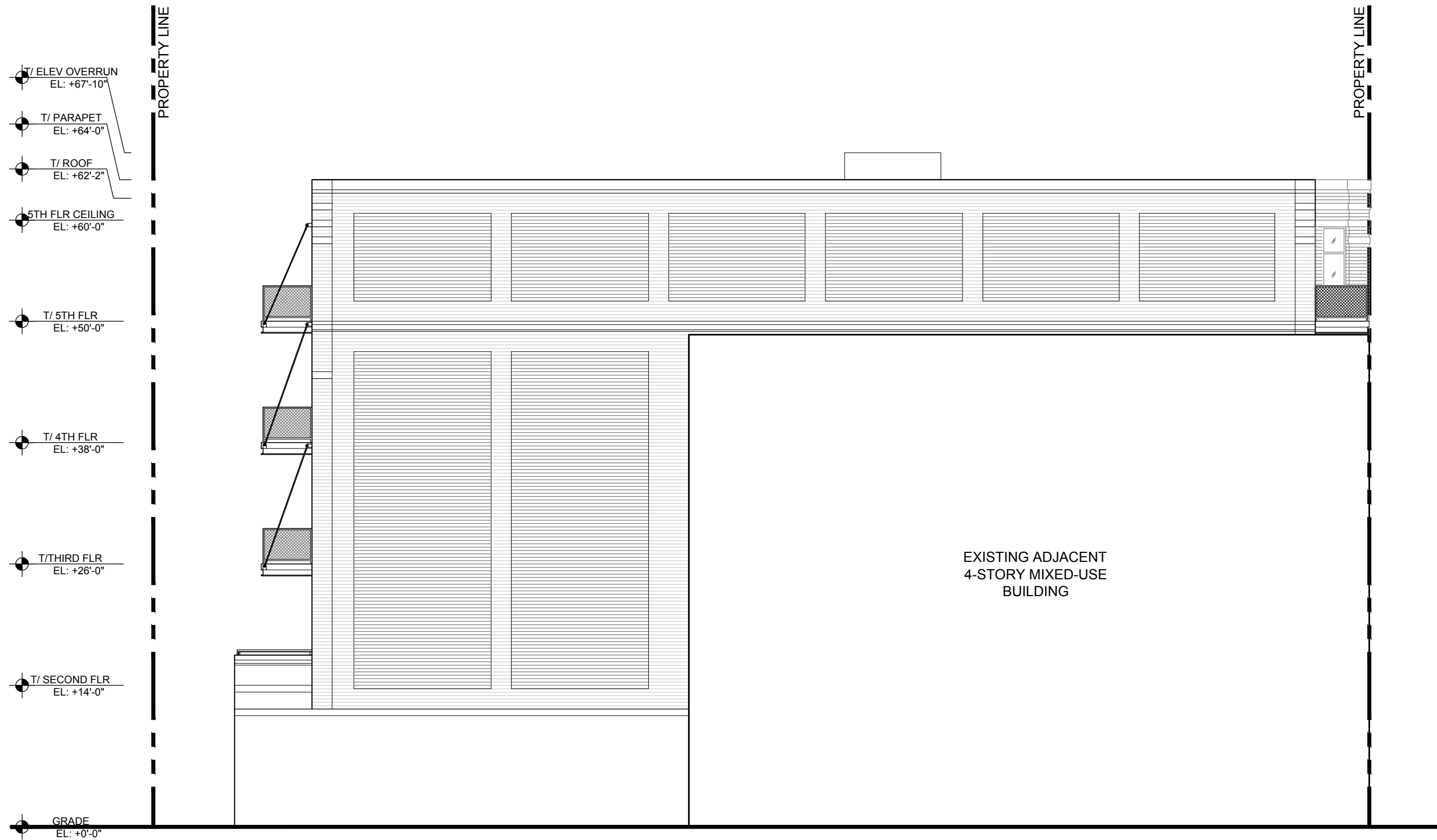
NORTH ELEVATION
