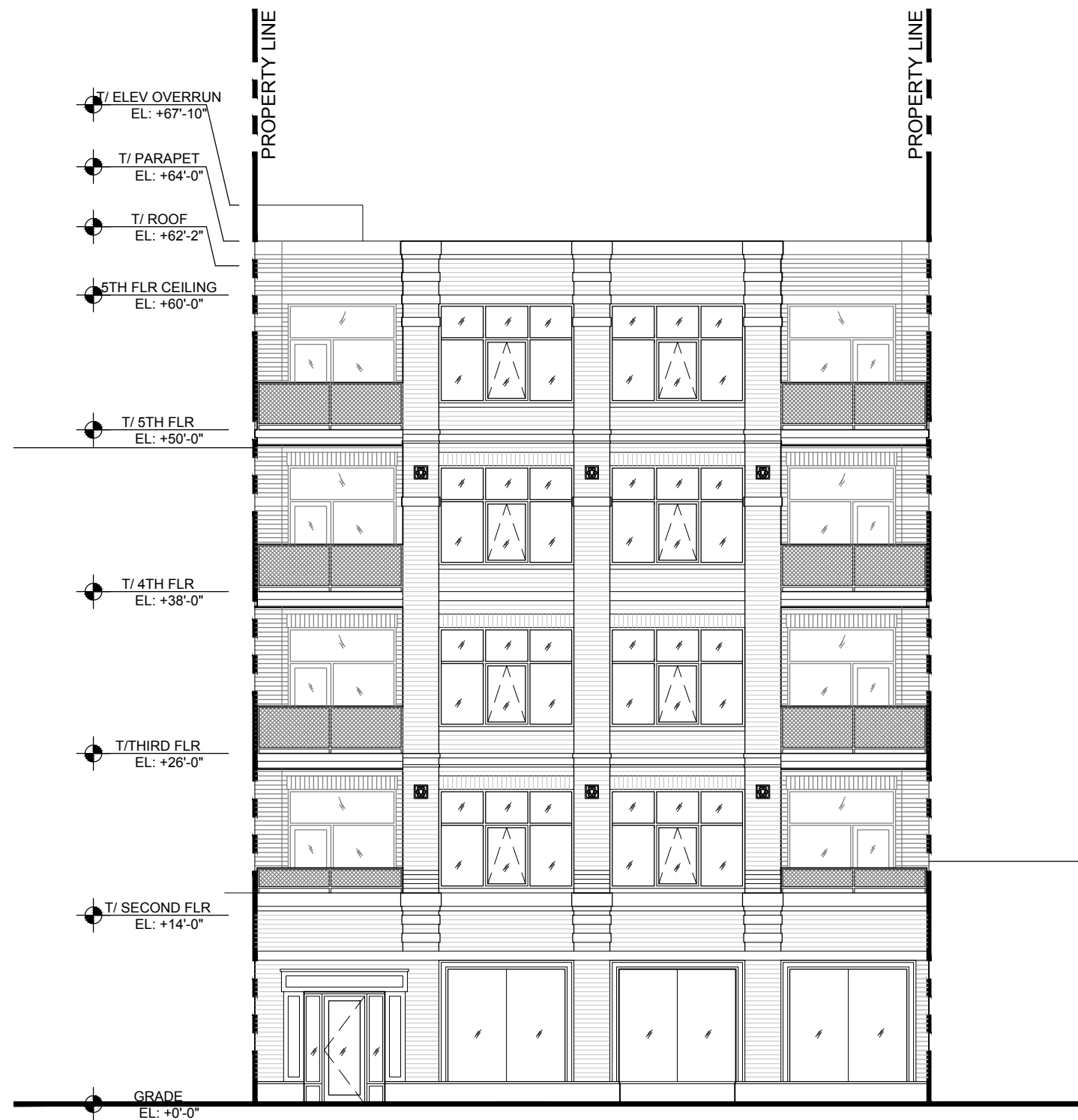
WEST ELEVATION
